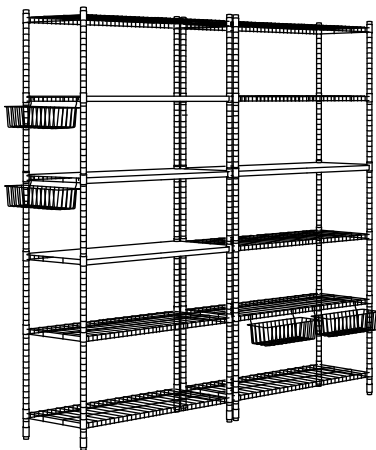
OMAR 2-section shelving unit Galvanized. Overall size: 77½×14½×71¼". This combination .96 892.790.51
