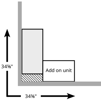
13 3/4" deep add-on unit for corner with one 29 1/2 x 13 3/4" frame.
