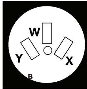
B) 3-wire wall receptacle (10-50R)
