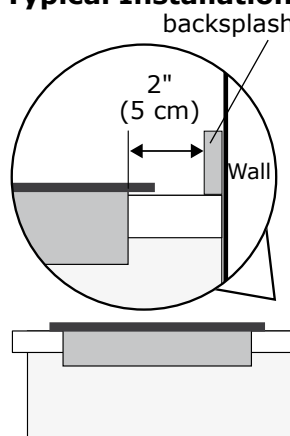
Figure 2c – Minimum Recommended Distance Between Rear Edge of Cutout and Nearest Combustible Surface Behind Countertop
