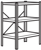
BROR shelving unit. Overall size: 85×55×110 cm.
