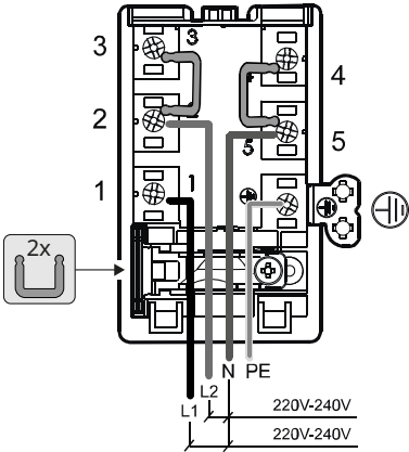
380 - 415 V ~ 2+N+GND
