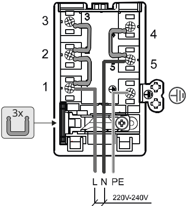
220 - 240V ~ 1+N+GND
