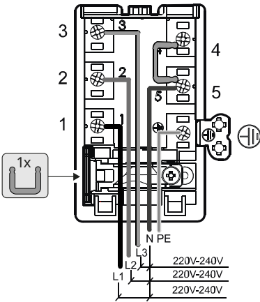
380 - 415V ~ 3+N+GND
