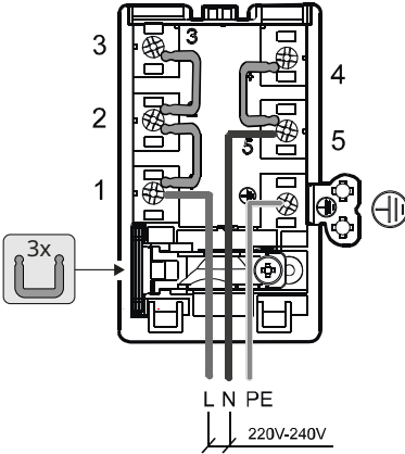
220 - 240V ~ 1+N+GND
