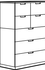
NORDLI chest of 7 drawers.* Total size: W80×D47×H122 cm White 992.395.02
