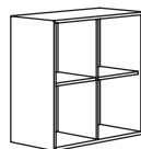
EKET cabinet with 4 compartments , 70×35×70 cm. Max. load 7 kg per shelf.
