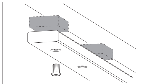
Detailed illustration of how to compensate the ceiling height with distance pieces.
