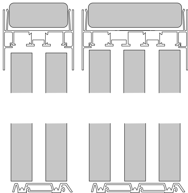
2-track rail with doors
