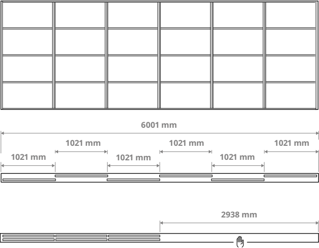
Combination with 6 doors and the 2-track rail. 6× 1021 mm doors
