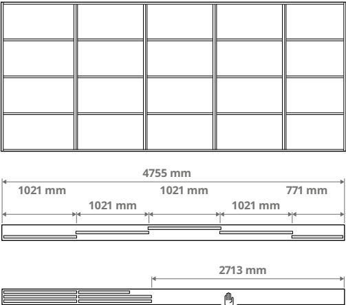
Combination with 5 doors and the 3-track rail. 1× 771 mm and 4× 1021 mm doors
