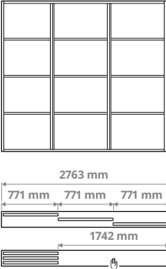
Combination with 3 doors and the 3-track rail. 1× 771 mm and 2× 1021 mm doors
