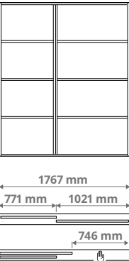
Combination with 2 doors and the 2-track rail 1× 771 mm and 1× 1021 mm door
