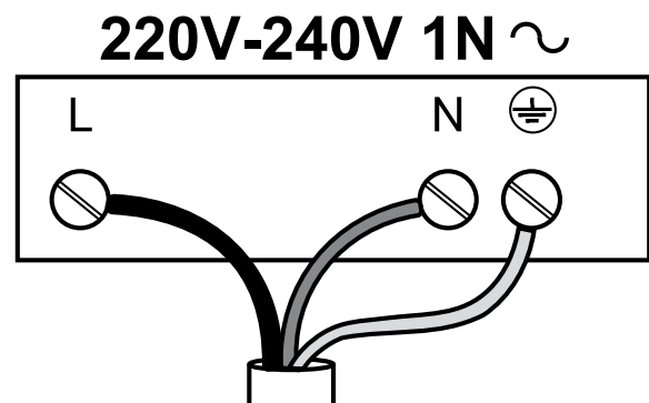
Connection diagram
