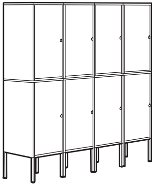
LIXHULT floor-based storage combination. Total size: W140×D35×H142 cm.
