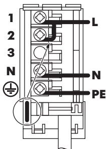
One-phase connection 220 V - 240 V ~
