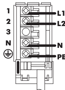
Two-phase connection 400 V 2L-1N ~
