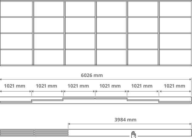
Combination with 6 doors and the 3-track rail. 6× 1021 mm doors
