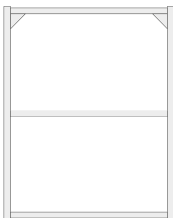
Étagère murale 30po (H76,2cm) Dimensions: 18×6po (L45,7×P15,2cm) 24×6po (L60,9×P15,2cm) 18×12po (L45,7×P30,4cm) 24×12po (L60,9×P30,4cm)
