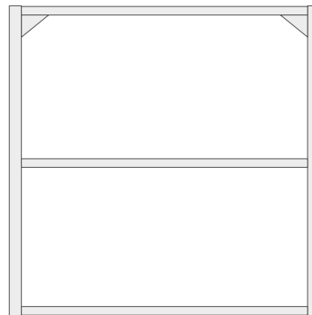
Base frame for sink with shelves H24" (60.9 cm) available in W24×D18" (60.9×45.7 cm)
