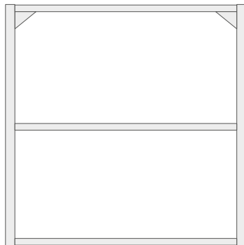
Base frame with shelves H24" (60.9 cm) available in W18×D18" (45.7×45.7 cm)
