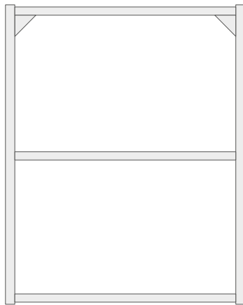
Wall frame with shelves H30" (76.2 cm) available in W18×D6" (45.7×15.2 cm) W24×D6" (60.9×15.2 cm) W18×D12" (45.7×30.4 cm) W24×D12" (60.9×30.4 cm)
