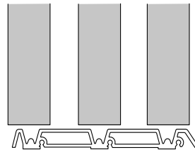
Sideview of 3-track rail with doors
