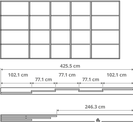
Combination with 5 doors and the 3-track rail. 3× 77.1 cm (30¾") and 2× 102.1 cm (40¼") doors, total width 425.5 cm (167½") , opening width 246.3 cm (97")
