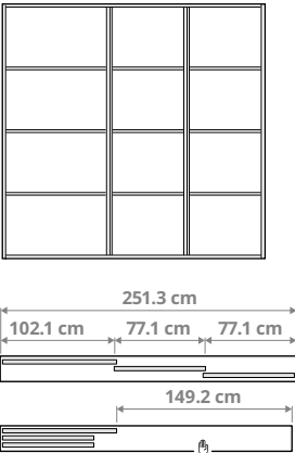
Combination with 3 doors and the 3-track rail. 2× 77.1 cm (30¾") and 1× 102.1 cm (40¼") doors, total width 251.3 cm (98¾") , opening width 149.2 cm (58¾")
