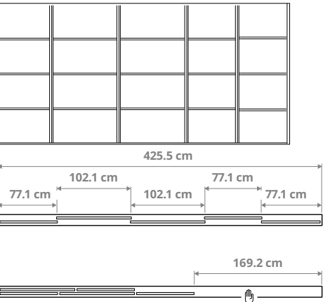
Combination with 5 doors and the 2-track rail. 3× 77.1 cm (30¾") and 2× 102.1 cm (40¼") doors, total width 425.5 cm (167½"), opening width 169.2 cm (66¾")
