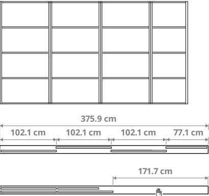
Combination with 4 doors and the 2-track rail. 1× 77.1 cm (30¾") and 3× 102.1 cm (40¼") doors total width 375.9 cm (148"), opening width 171.7 cm (67¾")
