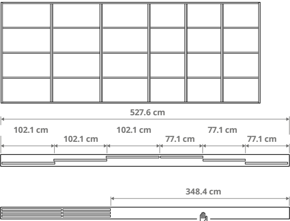
Combination with 6 doors and the 3-track rail. 3× 77.1 cm (30¾") and 3× 102.1 cm (40¼") doors, total width 527.6 cm (207¾") , opening width 348.4 cm (137¾")
