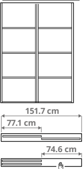
Combination with 2 doors and the 2-track rail 2× 77.1 cm (30¾") doors, total width 151.7 cm (59¾"), opening width 74.6 cm (29¾")
