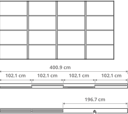
Combination with 4 doors and the 2-track rail. 4× 102.1 cm (40¼") doors, total width 400.9 cm (157⅞"), opening width 196.7 cm (77½")
