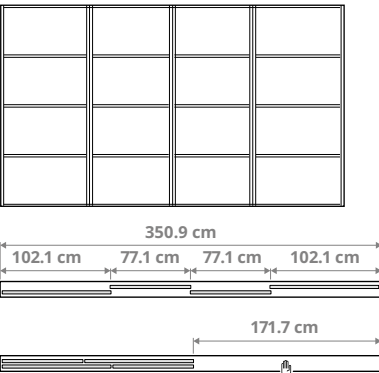
Combination with 4 doors and the 2-track rail. 2×77.1 cm (30¾") and 2× 102.1 cm (40¼") doors, total width 350.9 cm (138¾"), opening width 171.7 cm (67¾")
