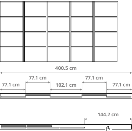
Combination with 5 doors and the 2-track rail. 4× 77.1 cm (30¾") and 1× 102.1 cm (40¼") doors, total width 400.5 cm (157¾"), opening width 144.2 cm (56¾")
