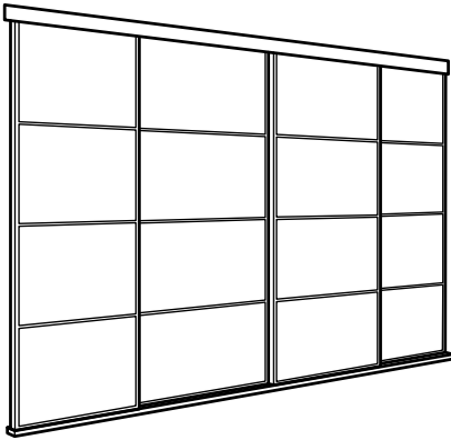
Combination with 4 doors and 2-track rail. 2× 77 cm (30 3/8") and 2× 102 cm (40 1/8") doors. SKYTТА/SVARTISDAL sliding door combination, white paper effect glass. Available in two heights. Overall size: 351×205 cm (138 1/4×80 3/4") (294.227.40) Overall size: 351×240 cm (138 1/4×94 1/2") (694.240.49)
