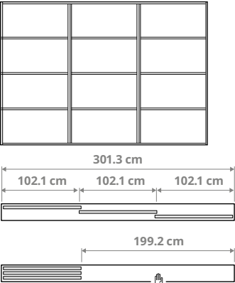
Combination with 3 doors and the 3-track rail. 3× 102.1 cm (40¼") doors, total width 301.3 cm (118¾") , opening width 199.2 cm (78¾")
