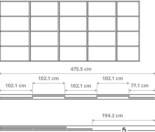
Combination with 5 doors and the 2-track rail. 1× 77.1 cm (30¾") and 4× 102.1 cm (40¼") doors, total width 475.5 cm (187¼"), opening width 194.2 cm (76½")
