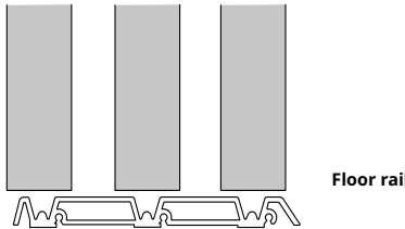
Sideview of 3-track rail with doors
