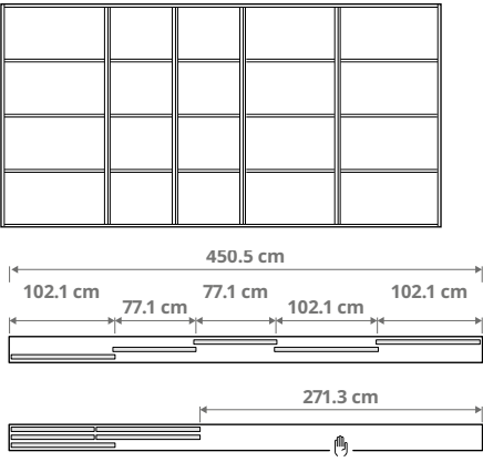
Combination with 5 doors and the 3-track rail. 2× 77.1 cm (30¾") and 3× 102.1 cm (40¼") doors, total width 450.5 cm (177¾") , opening width 271.3 cm (106¾")
