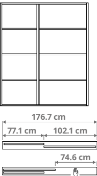
Combination with 2 doors and the 2-track rail 1× 77.1 cm (30¾") and 1× 102.1 cm (40¼") doors, total width 176.7 cm (69¾"), opening width 74.6 cm (29¾")
