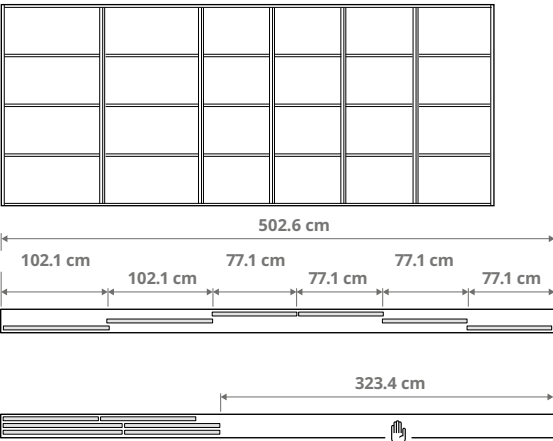
Combination with 6 doors and the 3-track rail. 4× 77.1 cm (30¾") and 2× 102.1 cm (40¼") doors, total width 502.6 cm (197¾") , opening width 323.4 cm (127¾")
