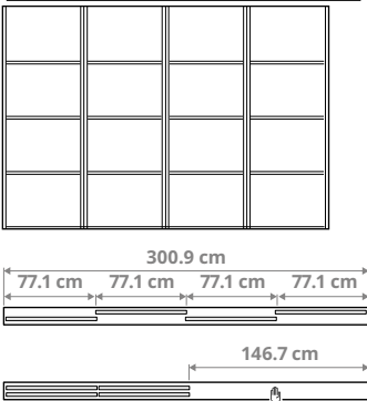
Combination with 4 doors and the 2-track rail 4× 77.1 cm (30¾") doors, total width 300.9 cm (118½"), opening width 146.7 cm (57¾")
