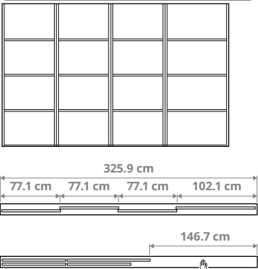
Combination with 4 doors and the 2-track rail 3× 77.1 cm (30¾") and 1× 102.1 cm (40¼") doors, total width 325.9 cm (128¾"), opening width 146.7 cm (57¾")
