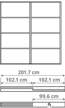
Combination with 2 doors and the 2-track rail 2× 102.1 cm (40¼") doors, total width 201.7 cm (79¾"), opening width 99.6 cm (39¾")
