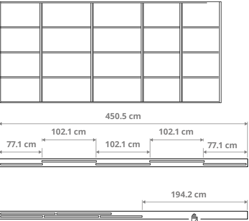
Combination with 5 doors and the 2-track rail. 2× 77.1 cm (30¾") and 3× 102.1 cm (40¼") doors, total width 450.5 cm (177¾"), opening width 194.2 cm (76½")
