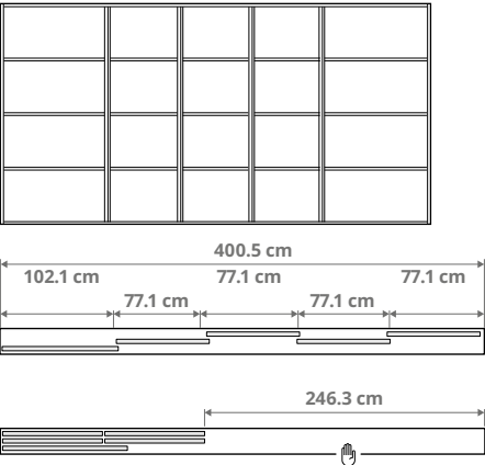
Combination with 5 doors and the 3-track rail. 4× 77.1 cm (30¾") and 1× 102.1 cm (40¼") doors, total width 400.5 cm (157¾") , opening width 246.3 cm (97")
