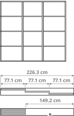
Combination with 3 doors and the 3-track rail. 3× 77.1 cm (30¾") doors, total width 226.3 cm (89¾") , opening width 149.2 cm (58¾")
