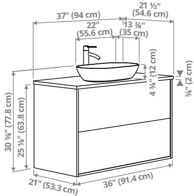
ÄNGSJÖN/OXMYREN vanity with drawers/sink/faucet, 37×21½×30⅜” (94×54.6×77.8cm).
