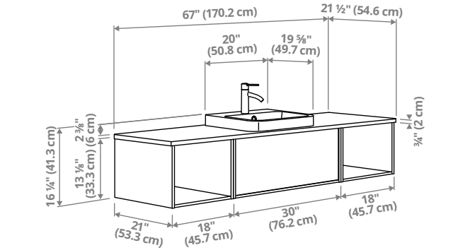
ÄNGSJÖN/BACKSJÖN vanity with drawers/sink/faucet, 67×21½×16¼" (170.2×54.6×41.3cm).
