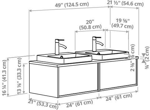
ÄNGSJÖN/BACKSJÖN vanity with drawers/sinks/faucets, 49×21½×16¼" (124.5×54.6×41.3cm).
