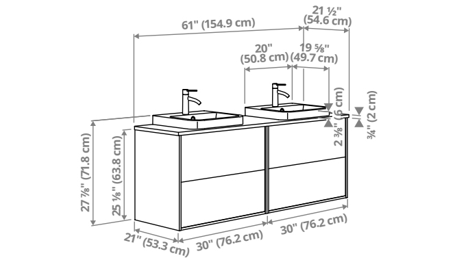
ÄNGSJÖN/BACKSJÖN vanity with drawers/sinks/faucets, 61×21½×28¼" (154.9×54.6×71.8cm).
