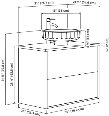
ÄNGSJÖN/LERSJÖN vanity with drawers/sink/faucet, 31×21½×31¾” (78.7×54.6×80cm).
