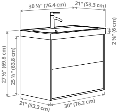
ÄNGSJÖN/BACKSJÖN vanity with drawers/sink/faucet, 30½×21×27½" (76.4×53.3×69.8cm).
