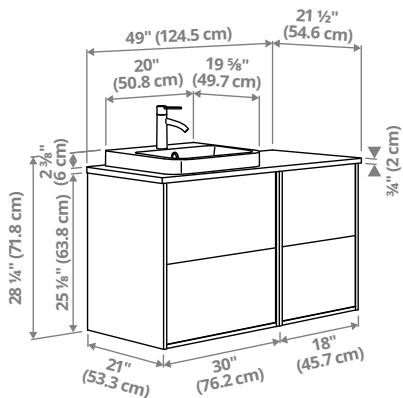
ÄNGSJÖN/BACKSJÖN vanity with drawers/sink/faucet, 49×21½×28¼” (124.5×54.6×71.8cm).
