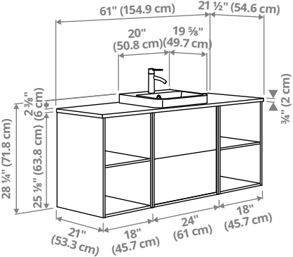
ÄNGSJÖN/BACKSJÖN vanity with drawers/sink/faucet, 61×21½×28¼" (154.9×54.6×71.8cm).
