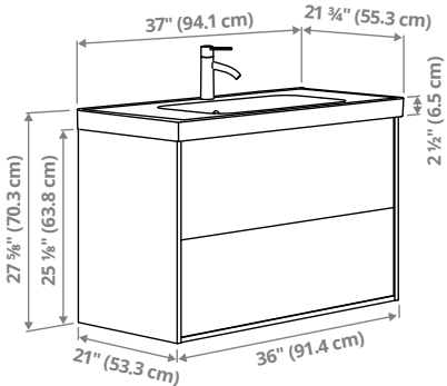
ÄNGSJÖN/ORRSJÖN vanity with drawers/sink/faucet, 37½×21¾×27½" (94.1×55.3×70.3).
