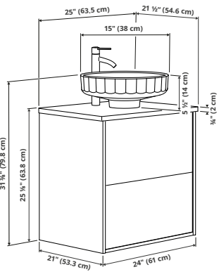
ÄNGSJÖN/LERSJÖN vanity with drawers/sink/faucet, 25×21½×31¾” (63.5×54.6×80cm).
