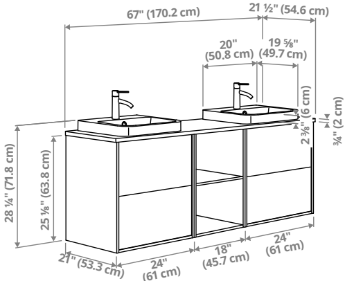
ÄNGSJÖN/BACKSJÖN vanity with drawers/sinks/faucets, 67×21½×28¼" (170.2×54.6×71.8cm).
