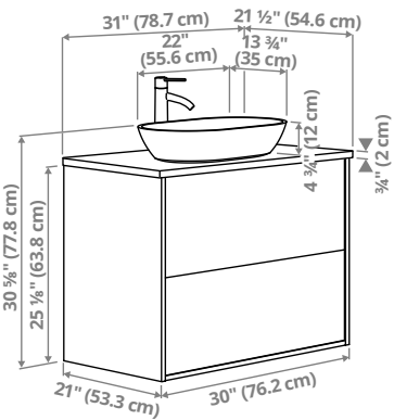
ÄNGSJÖN/OXMYREN vanity with drawers/sink/faucet, 31×21½×30⅜” (78.7×54.6×77.8cm).
