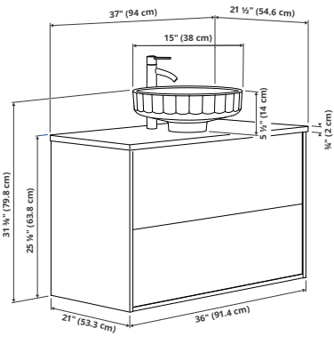
ÄNGSJÖN/LERSJÖN vanity with drawers/sink/faucet, 37×21½×31¾” (94×54.6×80cm).
