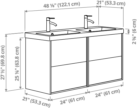
ÄNGSJÖN/BACKSJÖN vanity with drawers/sink/faucets, 48⅞×21×27½" (122.1×53.3×69.8cm).
