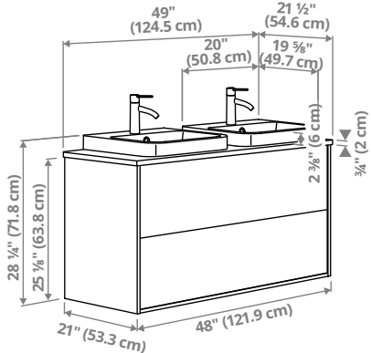
ÄNGSJÖN/BACKSJÖN vanity with drawers/sinks/faucets, 49×21½×28¼” (124.5×54.6×71.8cm).
