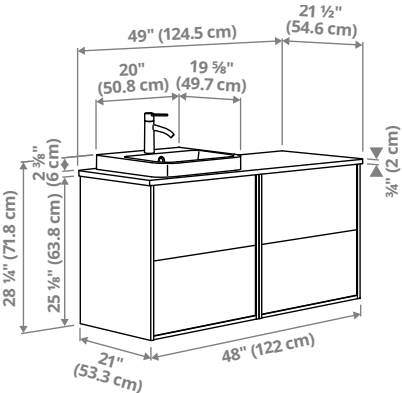
ÄNGSJÖN/BACKSJÖN vanity with drawers/sink/faucet, 49×21½×28¼" (124.5×54.6×71.8cm).
