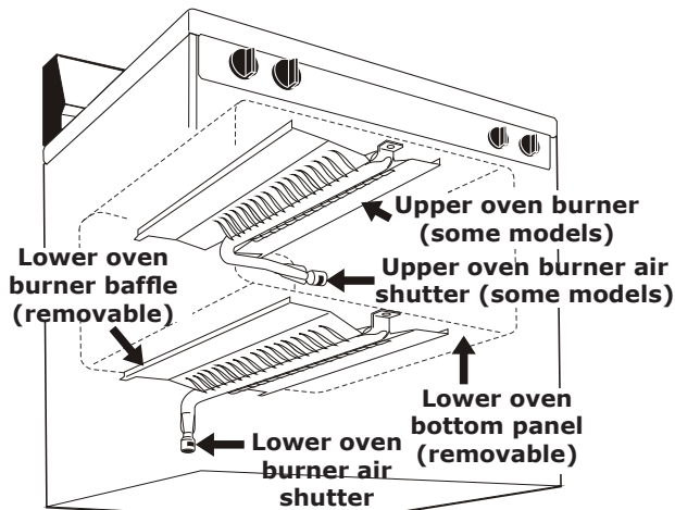
Fig. 19 - oven burner locations
