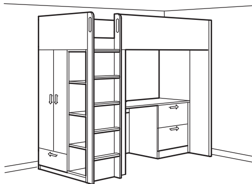
Loftbed combination with 2 drawers in the desk cabinet. Overall size: 206×104×182 cm Bed size: 90×200 cm
